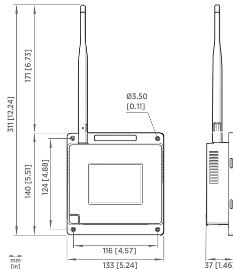
CA10 access point dimensions
